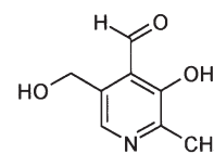
pyridoxal
