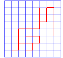
branched polymer
