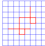
random walk
