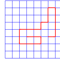
self-avoiding walk
